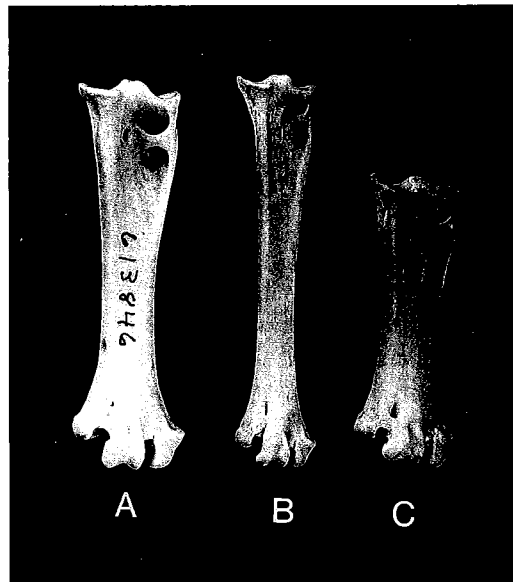
Fig. 5. Tarsometatarsi of Bubo in anterior view to show the great differences in proportions between various species. A, B. virginianus (USNM 613846); B, B. africanus (USNM 490288); C, B. sumatranus (USNM 559827). Figures three-fourths natural size.
